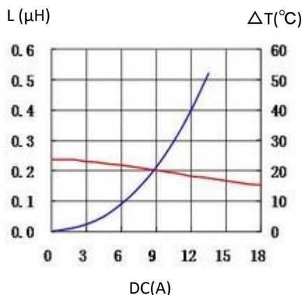
1. 0415CDMCCDS-R22MC
