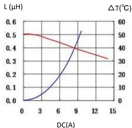
3. 0415CDMCCDS-R47MC
